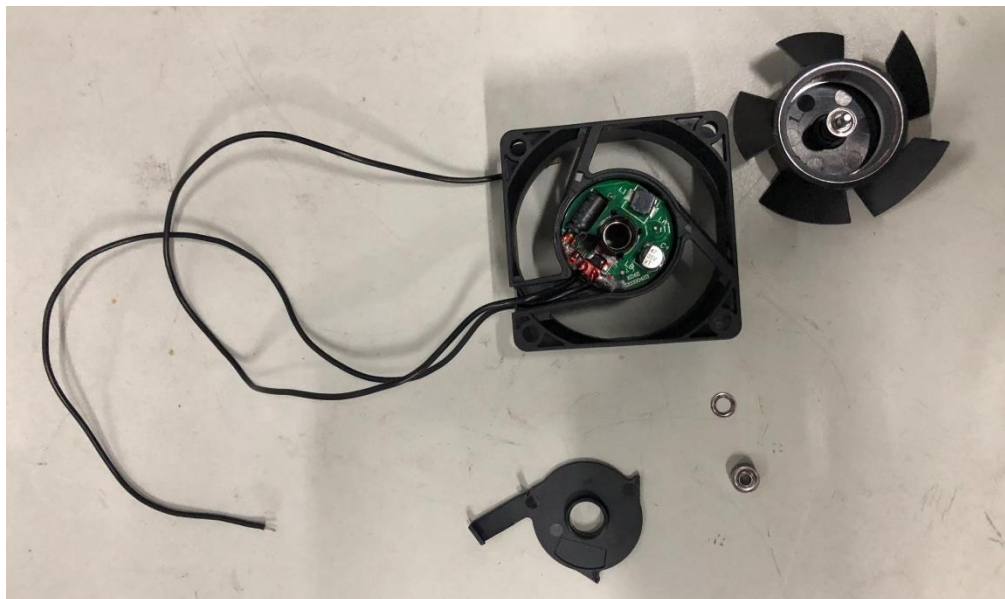
1#样品散件
